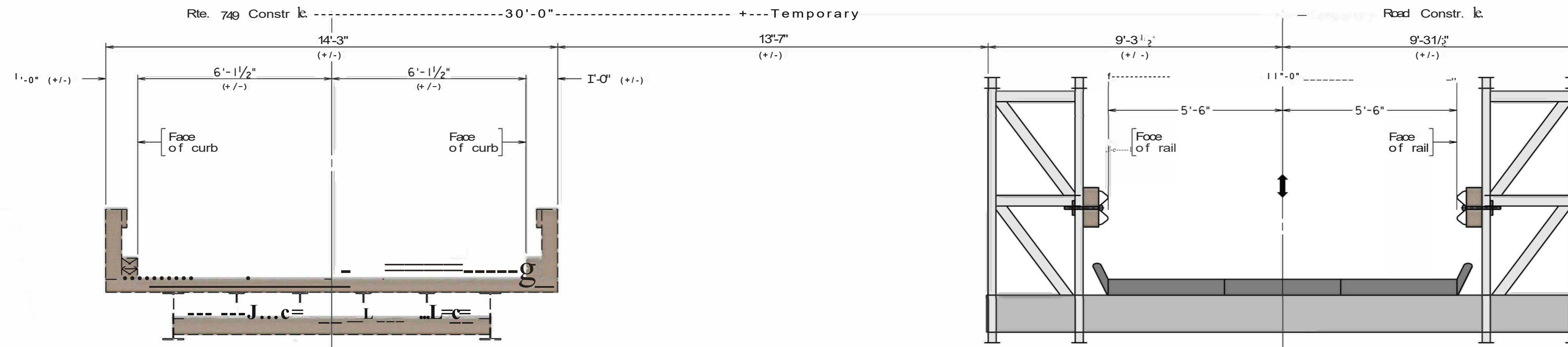
EXISTING WITH PHASE I TEMPORARY BRIDGE
